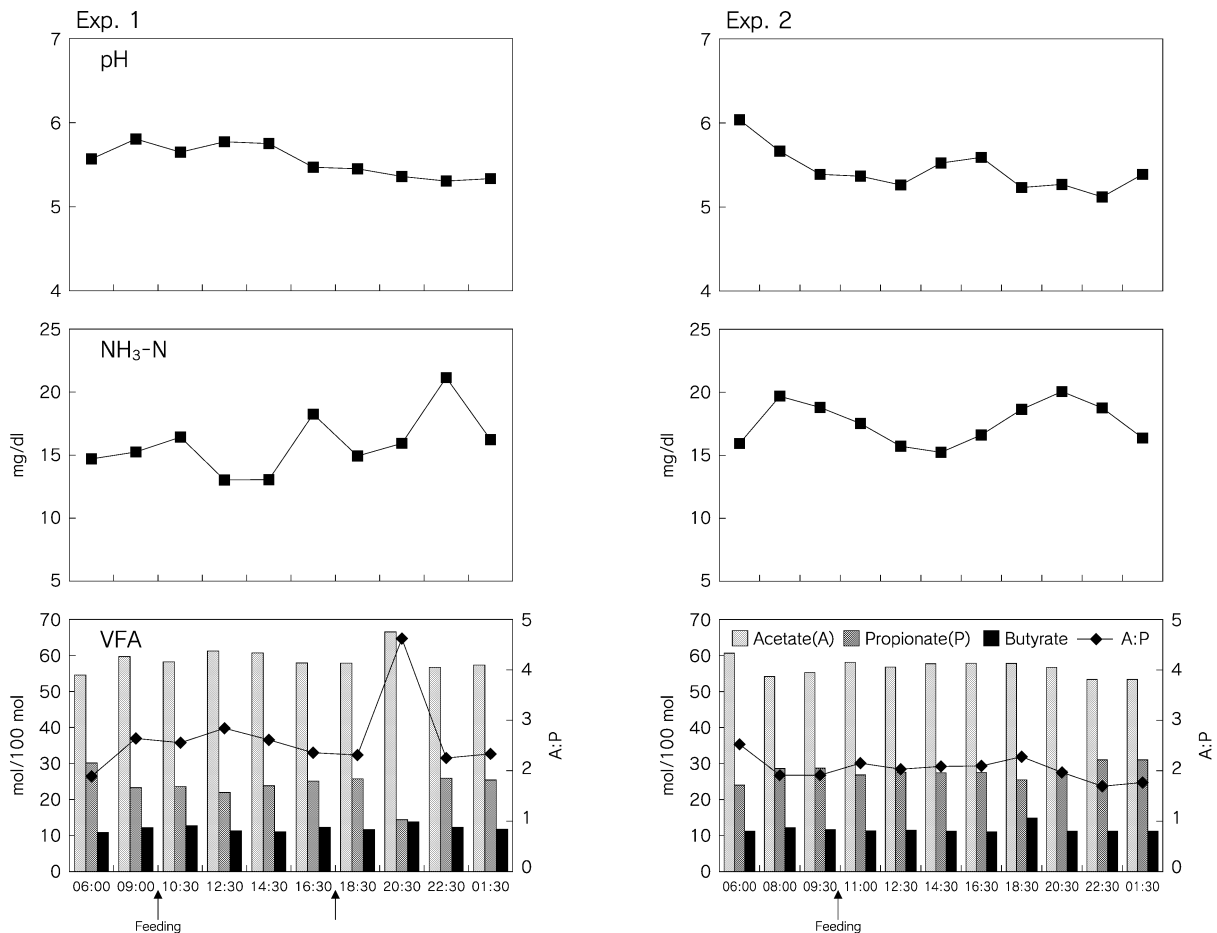
Figure 1. Diurnal changes in pH, NH 3 -N concentration and VFA molar percentages in rumen fluid from 2 cows.
